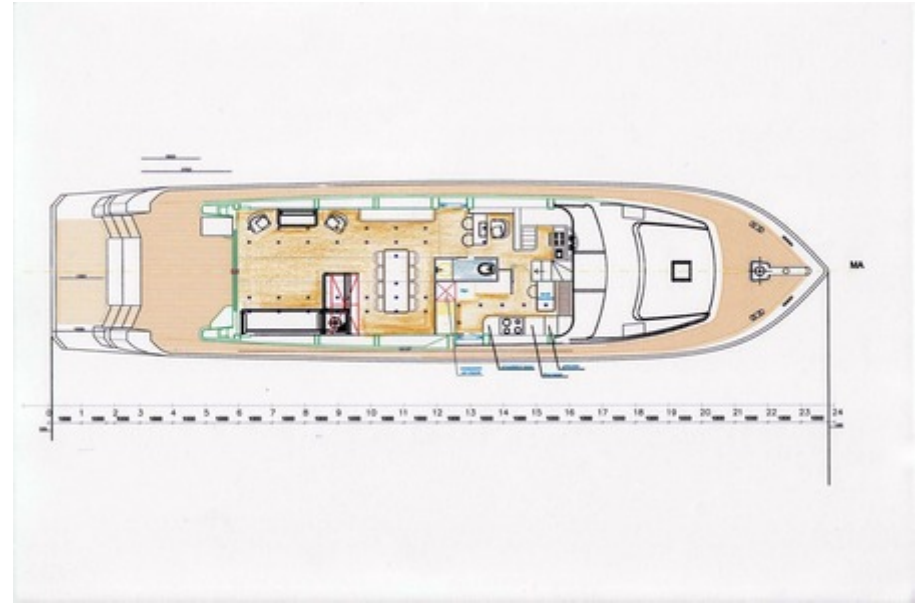
Main Deck Layout
